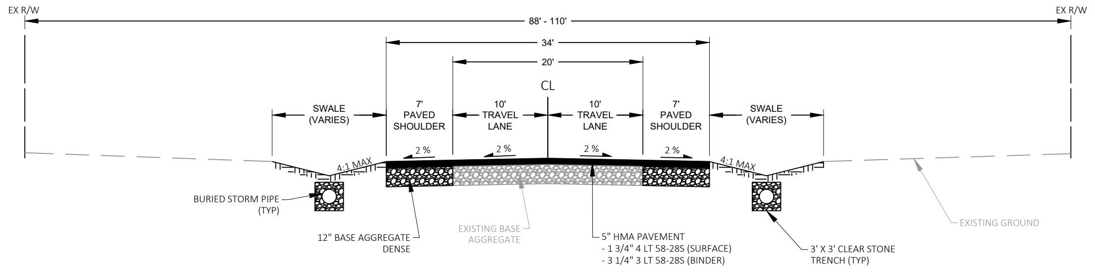
FINISHED TYPICAL SECTION BRADLEY ROAD ALTERNATE A
