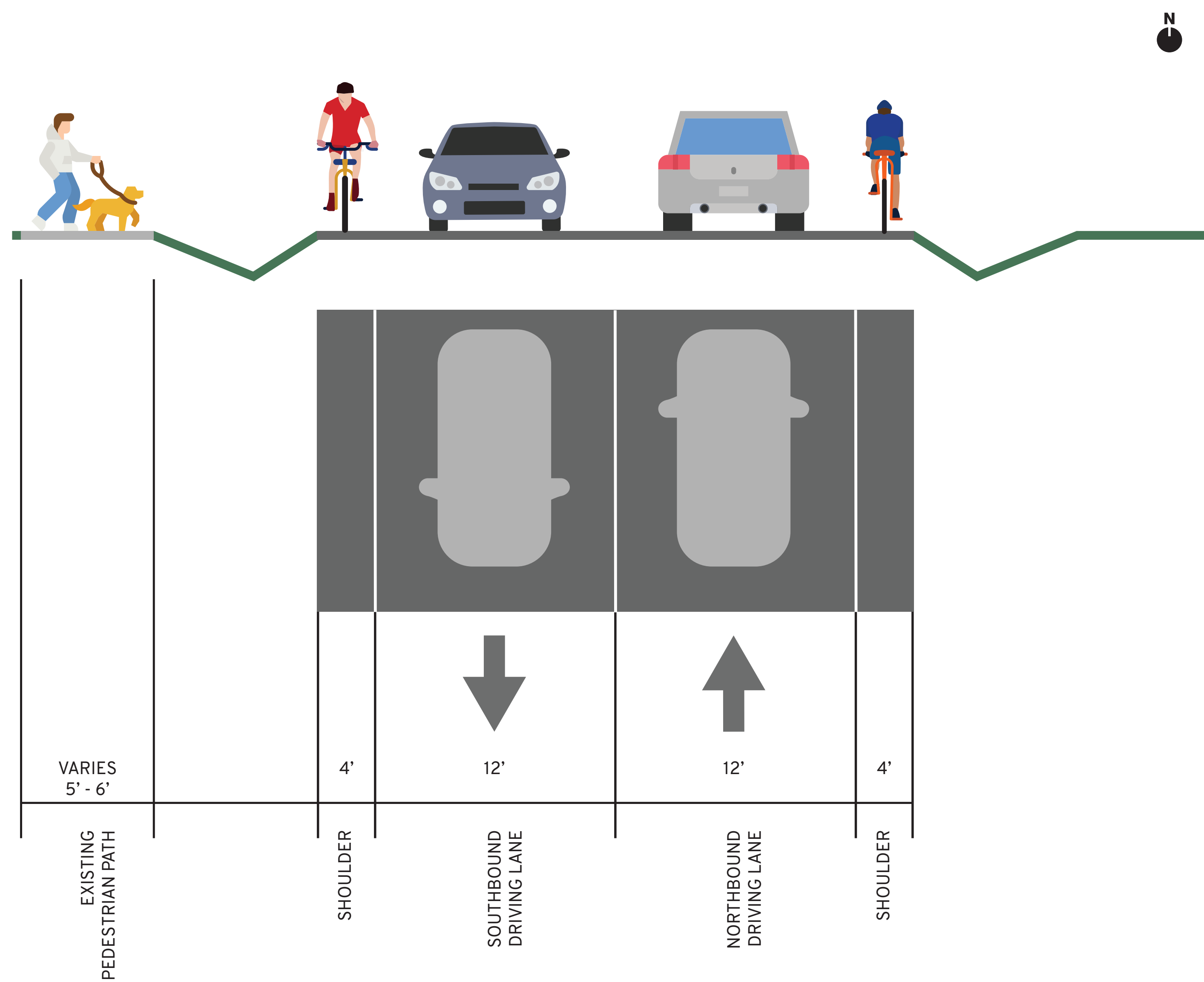
EXISTING TYPICAL SECTION
