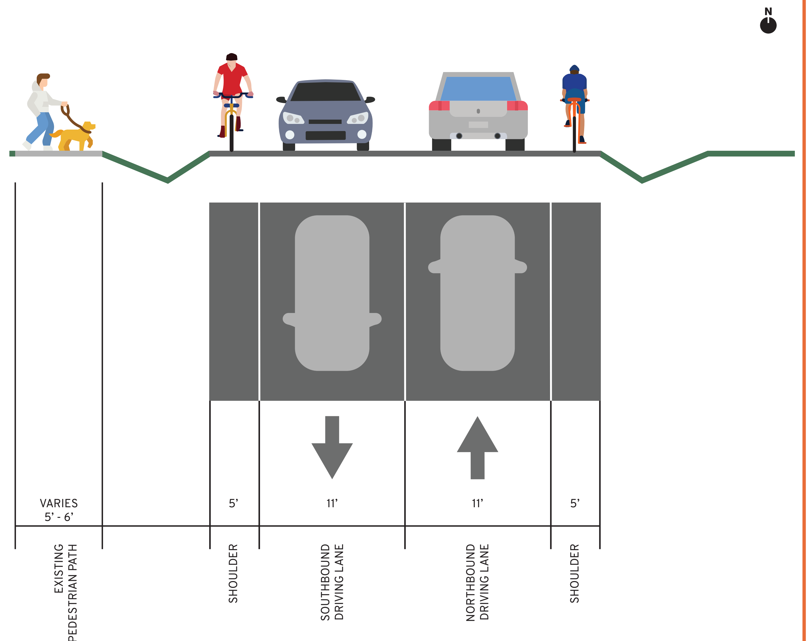
PROPOSED TYPICAL SECTION
